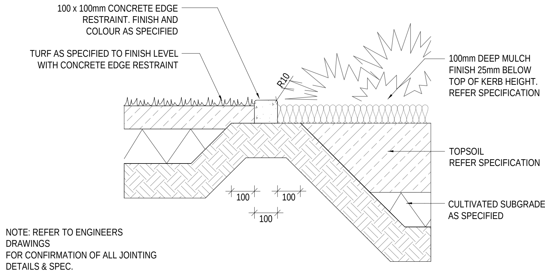
1 EDGE TYPE 1 - CONCRETE EDGE (TYPICAL) SCALE - 1 : 10
